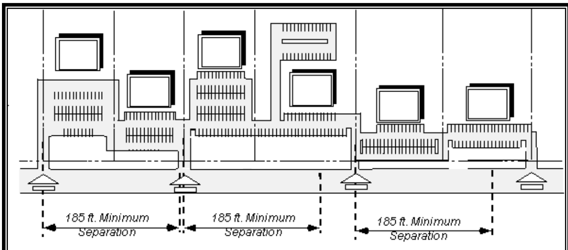
Minimum Driveway Separation at 40 mph Corridor Design Speed
